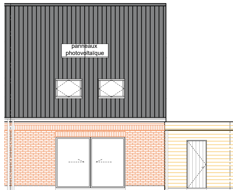
FACADE ARRIERE
